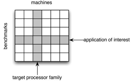
Figure 5: Cross-validation and leave-one-out setup: we eliminate the target machine and application of interest from the dataset when training the empirical performance models.
